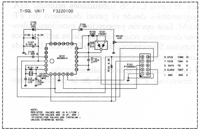
FTS-17A Circuit Diagram
